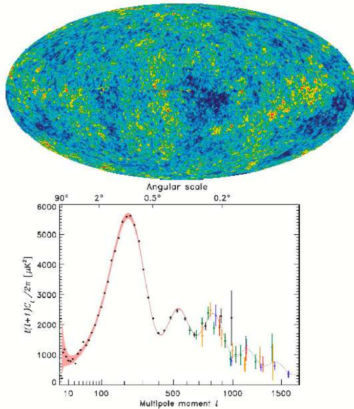
Cosmic microwave background
