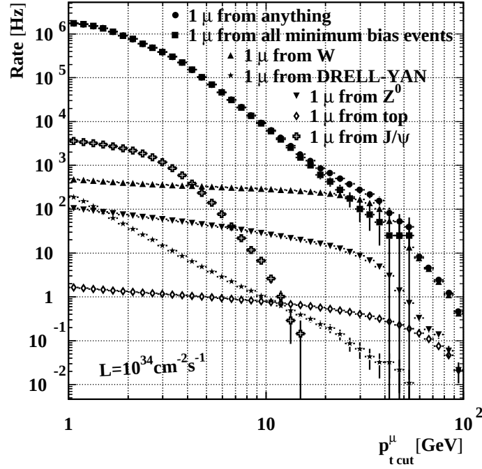
Figure 3.10: Single muon rates ( |\eta| < 2.4 ) [80]. The rate is defined as a number of events with at least one muon with transverse momentum p_t^\mu above a given threshold p_{tcut}^\mu .
