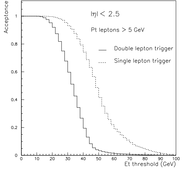
Figure 3.4: Acceptance of the single and double lepton trigger for H \rightarrow ZZ^* \rightarrow 4\ell ( m_H=120 GeV) [103].
