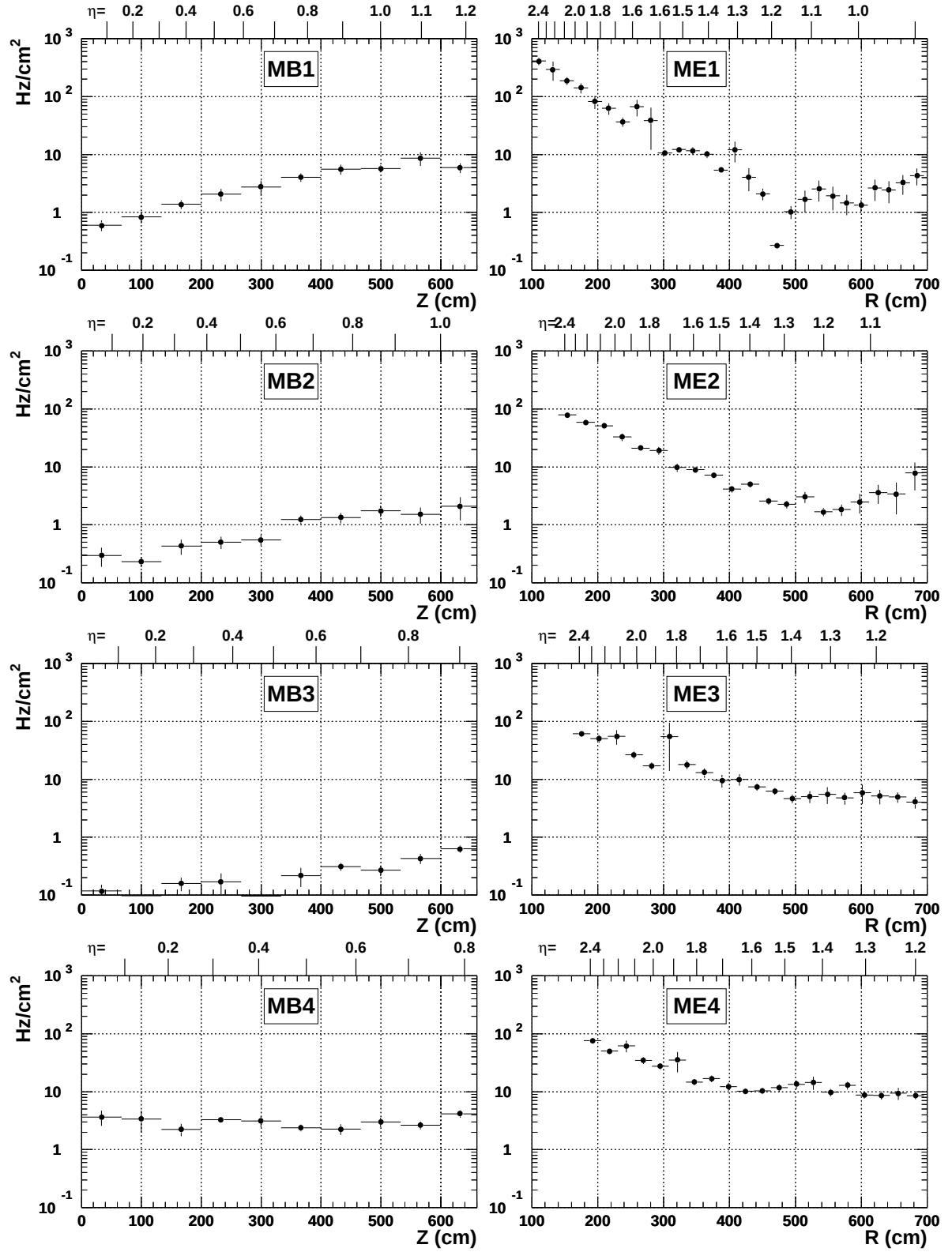
Figure 5.19: Total rate in muon chambers. Contributions of different kind of particles shown in Fig. 5.18 are summed together.
