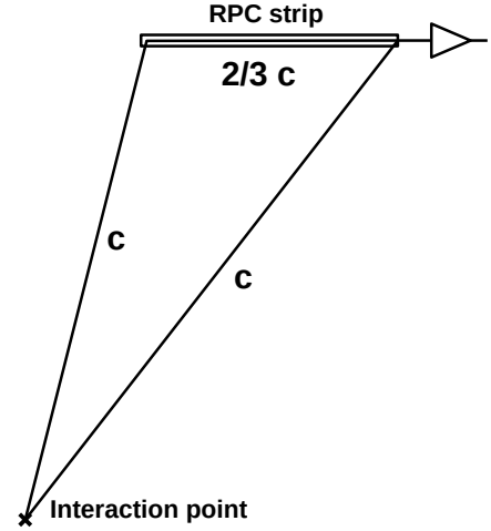
Figure 6.7: Uncertainty due to the time of flight and the signal propagation along the strip.
