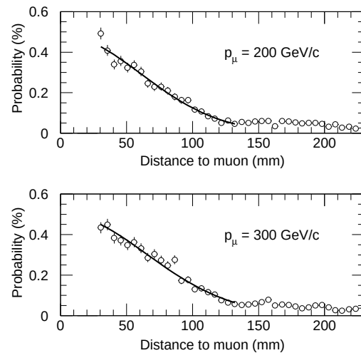
Figure 9.16: Measured (points) and simulated (lines) distance of secondary track from the muon. Track is defined as set of clusters in 4 CSC layers [152].
