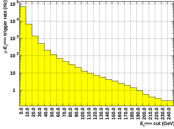
Figure 9.43: Muon- E_t trigger rate for p_t^{cut}(\mu) = 2\text{-}4\text{ GeV} at \mathcal{L} = 10^{33}\text{cm}^{-2}\text{s}^{-1} .
