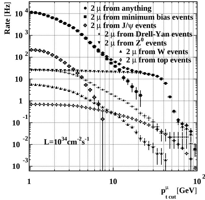
Figure 3.11: Double muon rates ( |\eta| < 2.4 ) [80]. The rate is defined as a number of events with at least two muon with transverse momentum p_t^\mu above a given threshold p_{tcut}^\mu . Notation “2 \mu from top events” means that at least one muon in each event comes from t or \bar{t} decay. The second one may come from another source, e.g. \pi or K decay.
