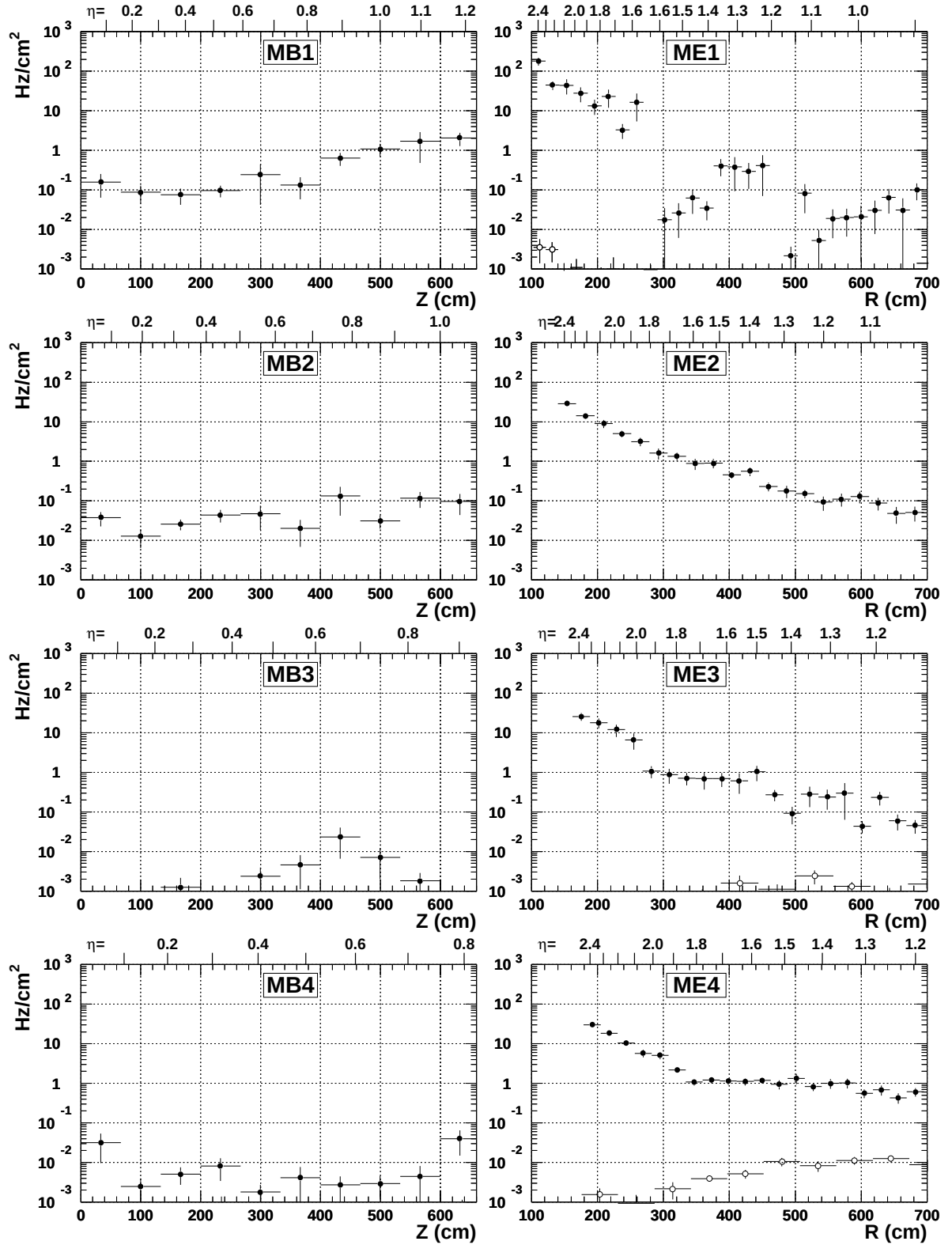
Figure 5.11: Charged hadron rates in the muon stations due to punchthrough and backsplashes of particles from pp interactions (full circles) [108] and from the beam halo (open circles) [114].
