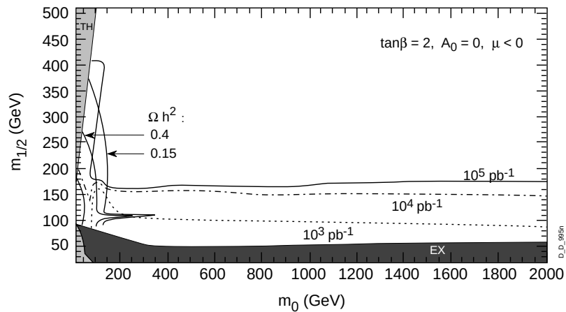
Figure 3.9: Expected observability of chargino and neutralino in \tilde{\chi}_i^{\pm} \tilde{\chi}_j^0 \rightarrow 3\ell + \cancel{E}_t + \text{no jets} [165]. The lines represent 5\sigma significance contours for different integrated luminosities. Relic neutralino matter density \Omega h^2 contours are also given. Shaded areas are excluded by theory (TH) or by previous experiments (EX).
