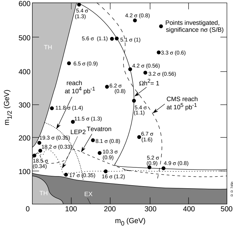
Figure 3.8: Expected observability of sleptons in 2 lepton final state in SUGRA MSSM with \tan\beta=2 , A_0=0 , \mu < 0 [164]. The dashed lines represent 5\sigma significance contours. The solid line represents cosmological \Omega h^2=1 boundary. Shaded areas are excluded by theory (TH) or by previous experiments (EX).
