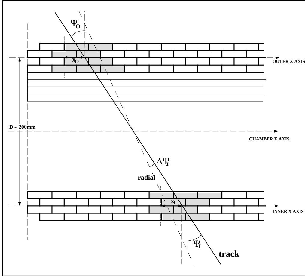
Figure 7.9: Track Correlator principle.
