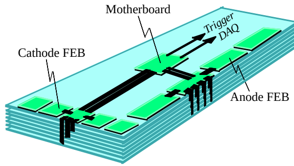
Figure 7.11: Front end electronics on CSC.
