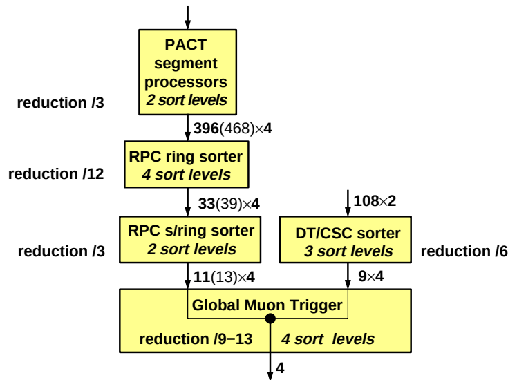
Figure 7.17: Muon Sorter tree.
