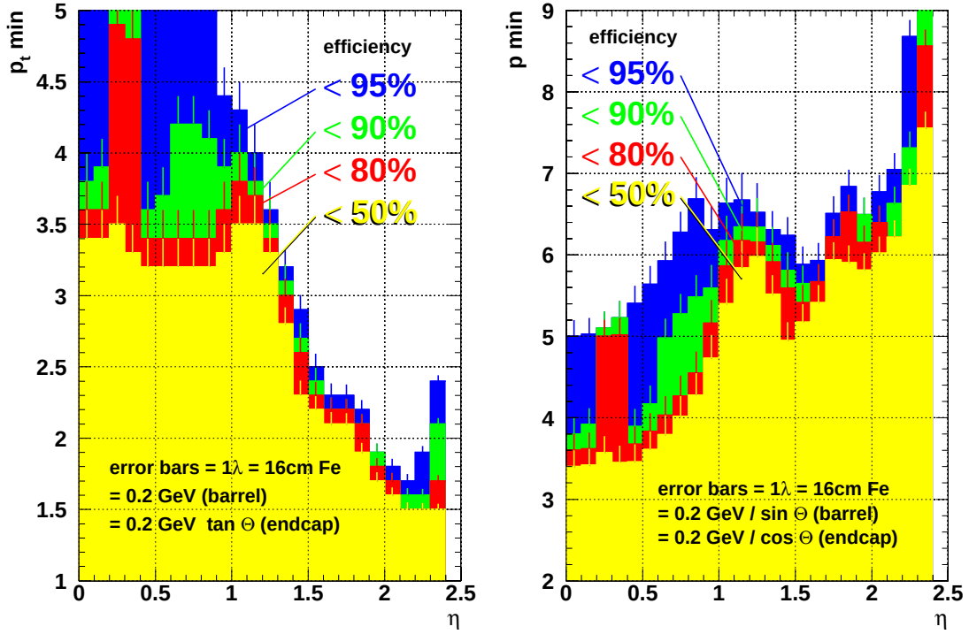
Figure 9.4: Minimal p_t and p thresholds for various efficiencies.
