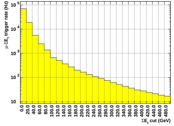
Figure 9.44: Muon- \Sigma E_t trigger rate for p_t^{cut}(\mu) = 2\text{-}4\text{ GeV} at \mathcal{L} = 10^{33}\text{cm}^{-2}\text{s}^{-1} .
