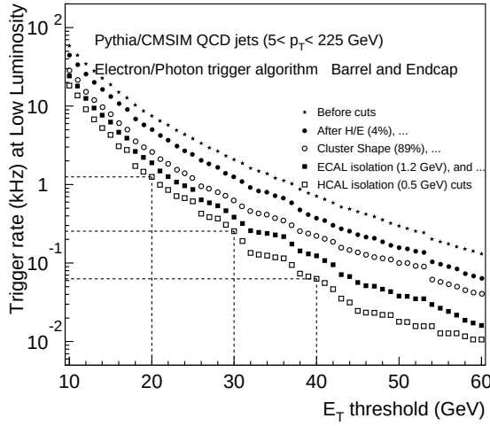
Figure 4.3: Single e/\gamma trigger rate [145]
