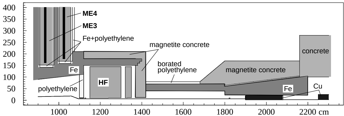
Figure 5.2: CMS shielding.
