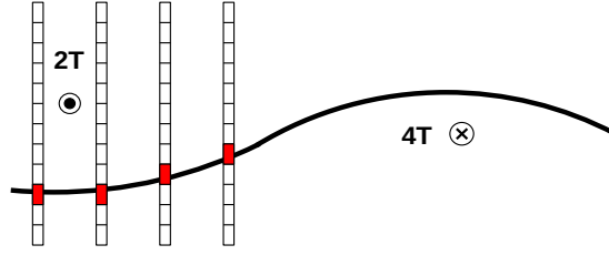
Figure 7.2: RPC Pattern Comparator Trigger principle.
